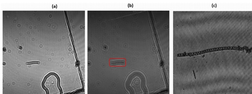
Filamentous algae (micro-plankton) (a) Digital hologram (b) Reconstructed image (c) Reconstructed image (zoomed and cropped from (b) )
