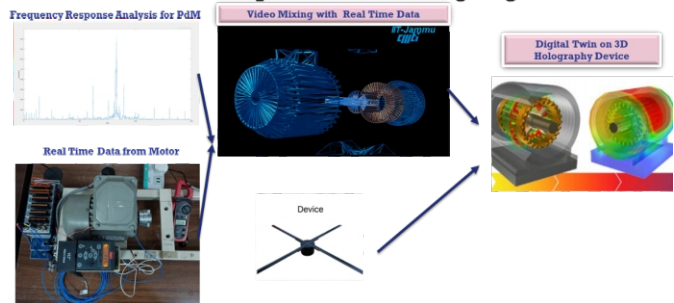
III. 3D Holography-based Digital Twin Framework- Induction Motor
