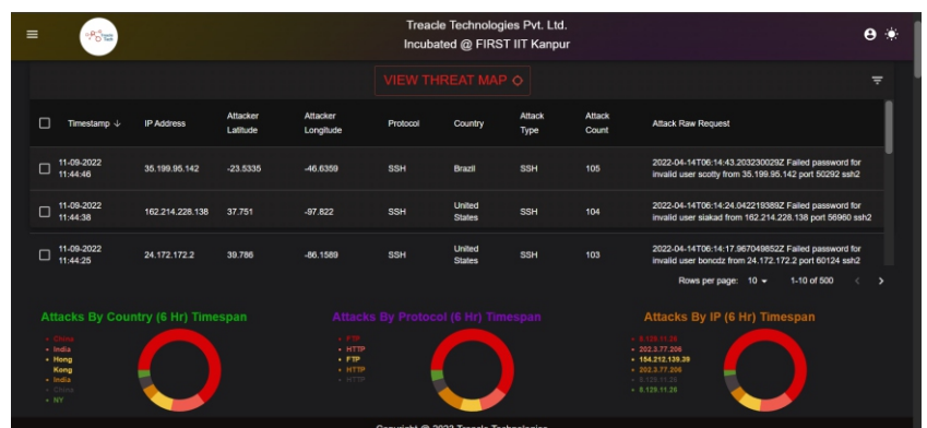
III. MUTACON Dashboard
