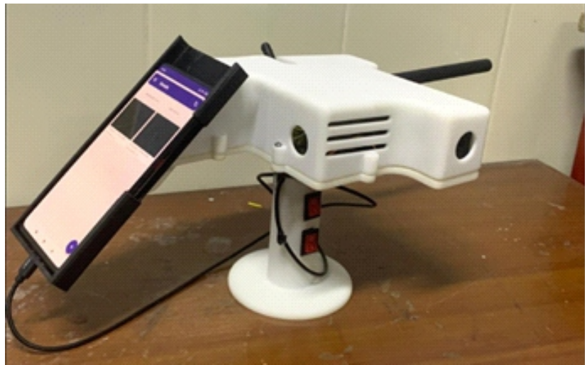
III. Smartphone Based Fluorescence Spectroscopy Device for Cervical Pre-cancer Detection
